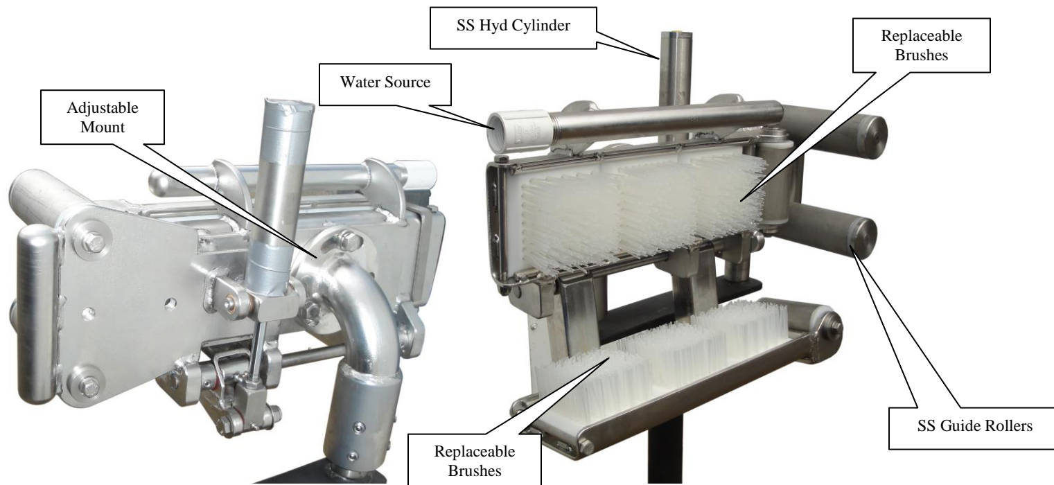
MODEL MFS03 Hydraulic-Operated Stainless Steel Fish Stripper/Hook Cleaner
